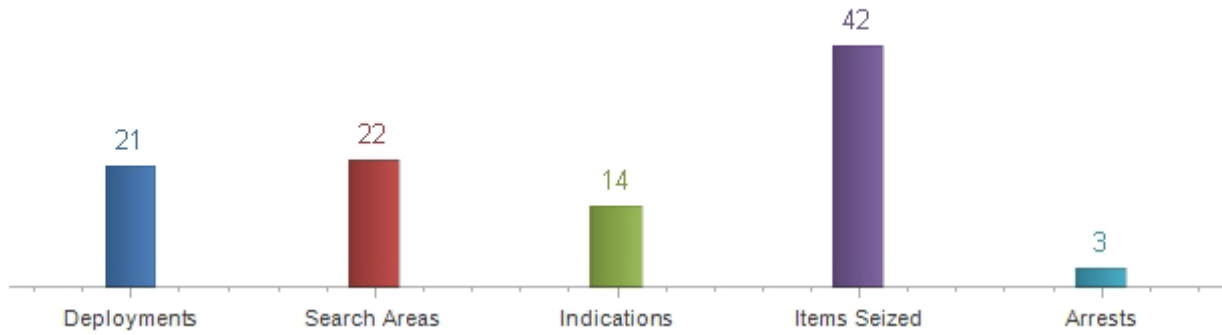
Detection Statistics
