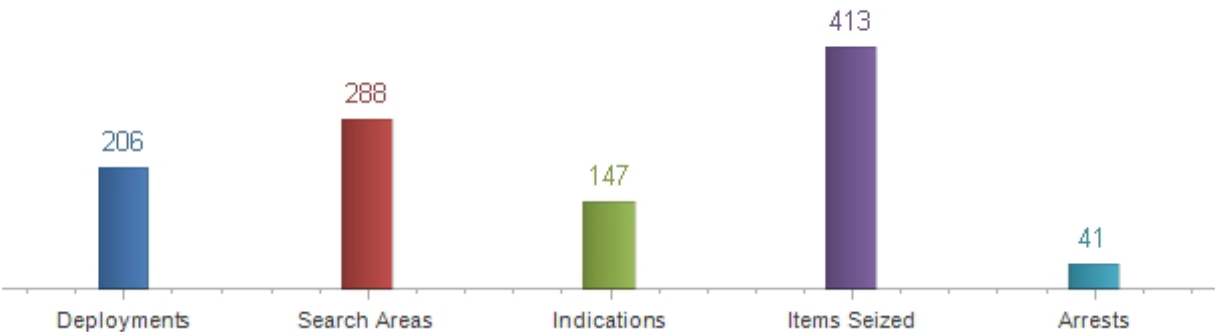
Detection Statistics
