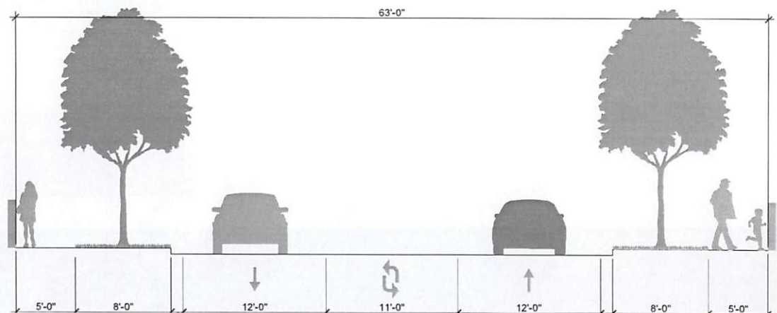
A.2 INTERSECTION ENTRY TYPICAL SECTION
