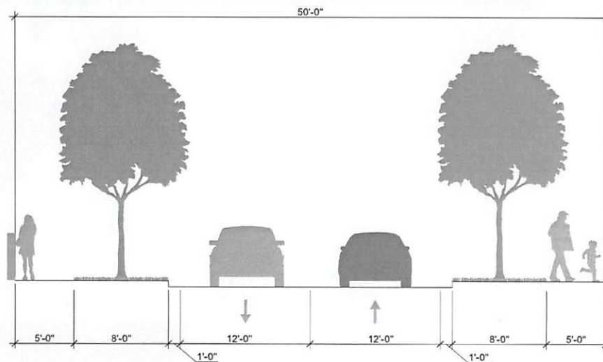
A.2 INTERSECTION ENTRY TYPICAL SECTION
